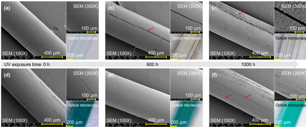
Fig. 2 Scanning electron microscopy (SEM) and optical microscopy were employed to analyse the samples (PA6 and PBSAT) before and after UV exposure. The arrows in Figures b and f denote longitudinal cracks, while the arrow in Figure c indicates extensive surface cracks. The ageing times for these samples were 0 hours (a,d), 600 hours (b,e), and 1000 hours (c,f). No discernible discoloration was observed in any of the samples, as evidenced by the insets in the optical microscopy images (Karl et al., ACS Applied Polymer Materials, 2025).
